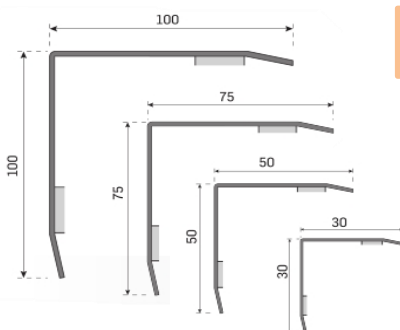
CCG(30S, 75S, 100S) Perfil de esquina en acero inoxidable Stainless steel corner profile
