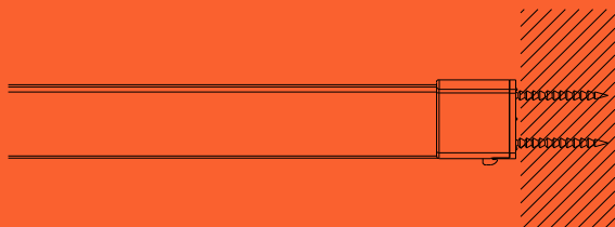
Support mural MTS
