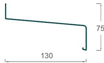
CCR050_606 15CMCCRNISA / PARAPET
