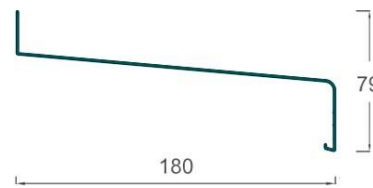
CCR051_606 20CMCCRNISA / PARAPET
